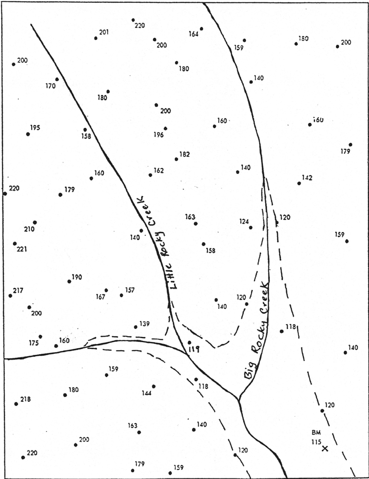
Elevation points for drawing a contour map.
